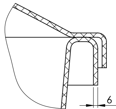
DETAIL A SCALE 1 : 2.5
