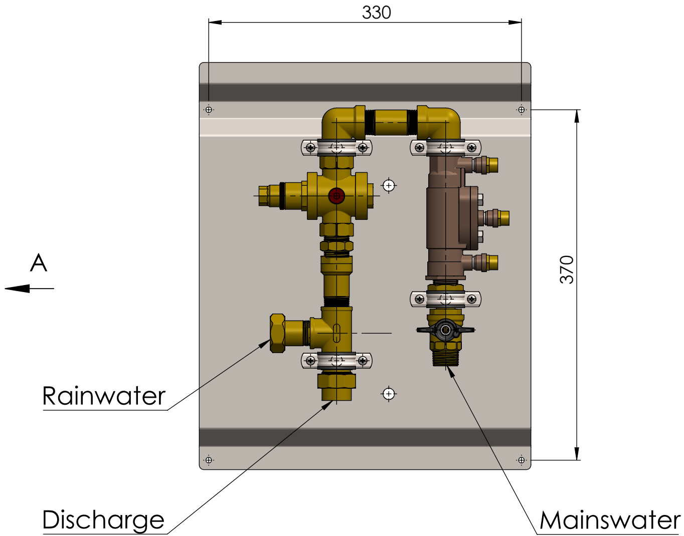
VIEW A Cover is not shown
